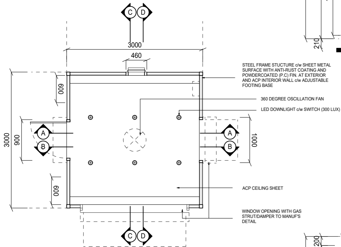
CEILING PLAN SCALE 1: 50
