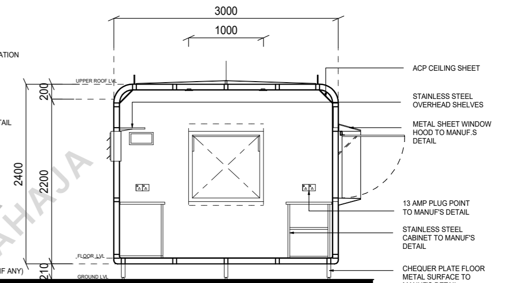
SECTION D - D SCALE 1: 50
